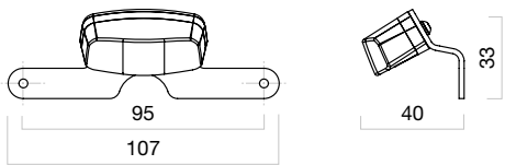
Rear Light with License Plate Light R 3356075 E ■ EE130B
