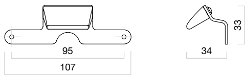
License plate support light (with bracket) R 1775172 E ■ EE091B
