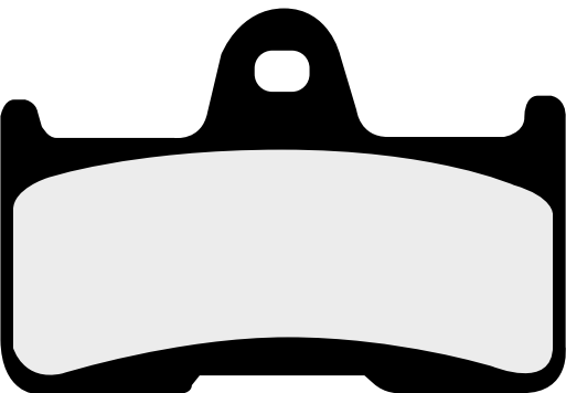
2P309 • 65,50 x 44,75 x 11,65mm
