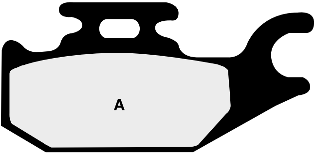
2P291 • A. 82,08 x 40,85 x 9,46mm / B. 62,03 x 40,80 x 9,46mm
