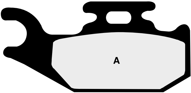
2P292 • A. 82,08 x 40,85 x 9,46mm / B. 62,03 x 40,80 x 9,50mm
