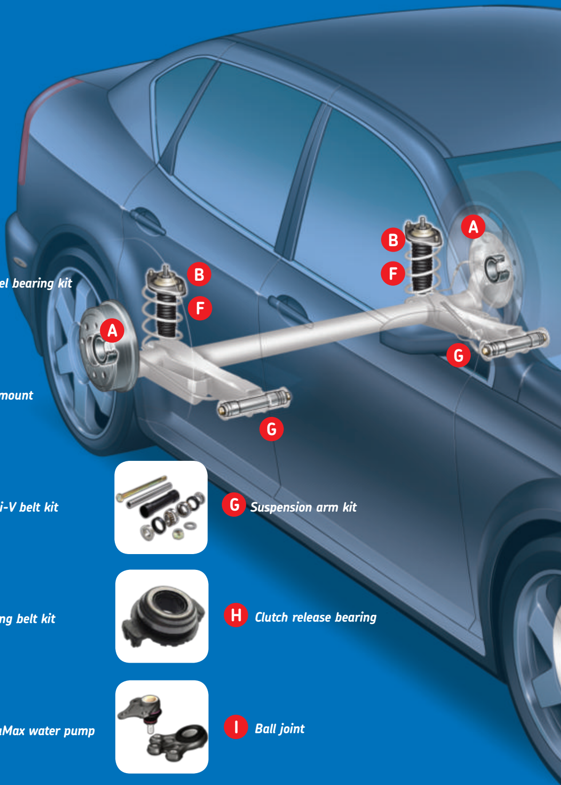
F Strut protection kit
