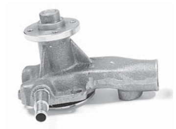
125-1340 1Paper Gasket
