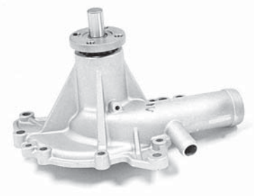
130-1070 1Paper Gasket
