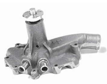
130-1260 1Paper Gasket, 1clamp, 1instruction, 1rubber plug
