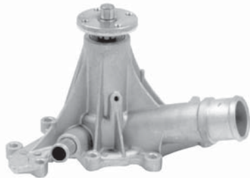
125-5055 1Paper Gasket
